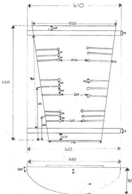
Plan of Testing Board (measurements in mm)
